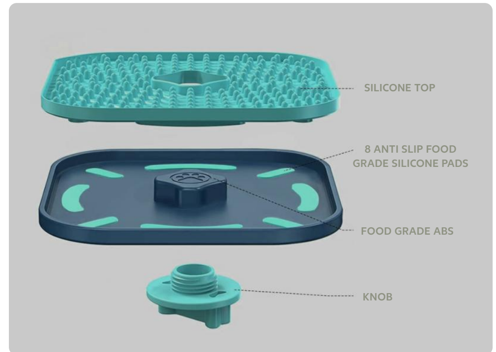
LICK MAT CAGE PROTOTYPE - 7" L X 7" W X 1.5" H
