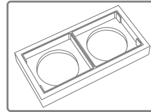
1. Pick leg from inside of the base
